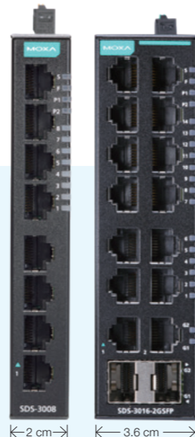
SDS-3008/3016 Series 8/16-port Smart Switches
