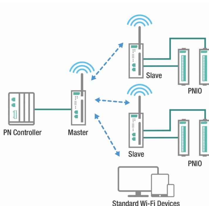
Figure 6-1. P2MP bridge supporting standard Wi-Fi devices using Moxa Master/Slave
